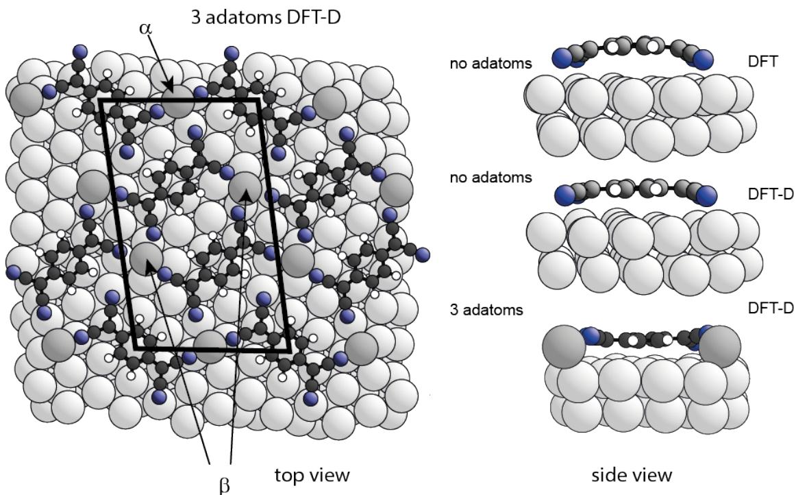
Fig. 3. Left: Top view of the DFT-D-optimised structural model of the TCNQ surface phase with three Ag adatoms per unit mesh (shown by the black lines). Notice that there are two symmetrically distinct Ag adatom sites in this model, labelled \alpha and \beta . Alternative models with 1, 2 or 3 Ag adatoms missing were also explored (Table 2). Right: Side views of a single molecule within the no-adatom model and in the 3-adatom model resulting from both DFT and DFT-D calculations. Ag adatoms are shaded darker than the substrate atoms. Other colours as in Fig. 1(a).
