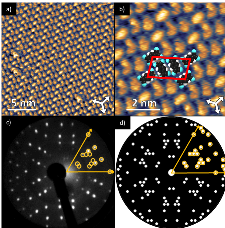
Fig. 1 (a & b) STM images at two different magnifications of the \begin{pmatrix} 2 & 5 \\ -8 & -2 \end{pmatrix} ordered phase formed by TCNQ on Ag(111) ( V_{\text{samp}} = -1.00 V, I = 55 pA). The substrate \langle 110 \rangle directions are indicated by the white arrows. Superimposed on (b) is the surface unit mesh and a schematic representation of the TCNQ molecules. H atoms are coloured white, N atoms blue, carbon atoms black. For larger area STM images see ESI † . (c) LEED pattern recorded at a kinetic energy of 14.5 eV. The location of the beams match those predicted for a \begin{pmatrix} 2 & 5 \\ -8 & -2 \end{pmatrix} commensurate matrix as shown in the simulated pattern (d) obtained using the LEEDpat program 37 , including the beams from the 6 symmetry-equivalent domains arising from the 3m symmetry of the substrate. The predicted beams in one sector of (c) are superimposed as open rings on the experimental pattern in (b). Yellow arrows correspond to the \langle 211 \rangle directions of the primitive translation vectors of the substrate unit mesh.
