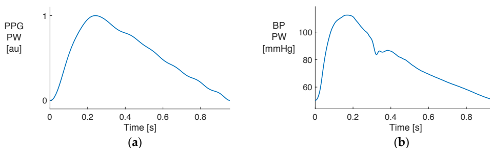
Figure 2. A comparison of (a) photoplethysmogram (PPG) and (b) blood pressure (BP) pulse waves.
