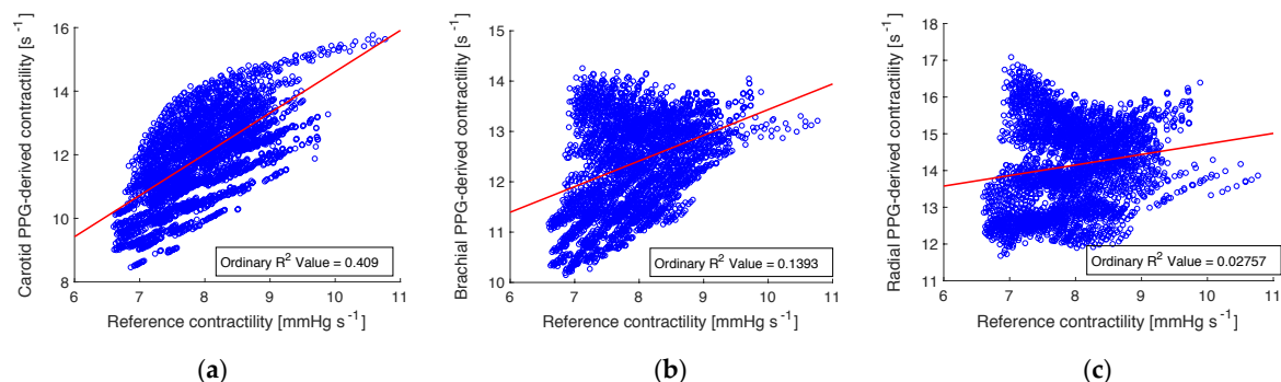
Figure 4. Estimating left ventricular contractility (LVC) from the PPG: the correlation between estimated at reference values at (a) the carotid artery ( i.e. neck); (b) the brachial artery ( i.e. upper arm); and (c) the radial artery ( i.e. wrist). Least-squares lines are shown in red.
