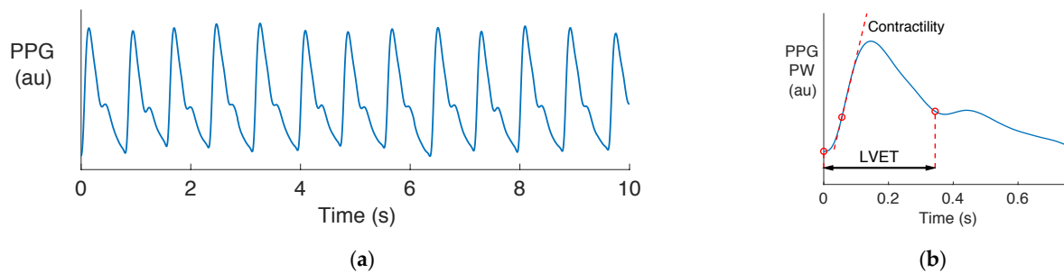
Figure 1. The photoplethysmogram (PPG) signal: (a) A 10 s in vivo recording of the PPG, exhibiting 12.5 pulse waves (PWs), one for each heart beat; (b) The techniques for estimating left ventricular ejection time (LVET) and left ventricular contractility (LVC) from a single PW. au: arbitrary units. Data from the Vortal dataset [12].
