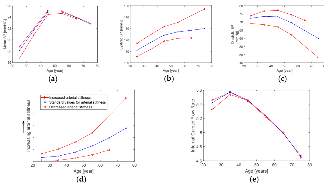
Figure 3. The simulated changes in risk factors for Alzheimer's Disease (AD). Changes in mean, systolic and diastolic blood pressure (BP) with age are shown in (a–c) respectively. The central blue lines indicate normal values for arterial stiffness at each age, upper red lines indicate increased stiffness, and lower red lines indicate lower stiffness. Reference arterial stiffness values are shown in (d), calculated from aortic pulse wave velocity. The changes in flow rate at the carotid artery are shown in (e).
