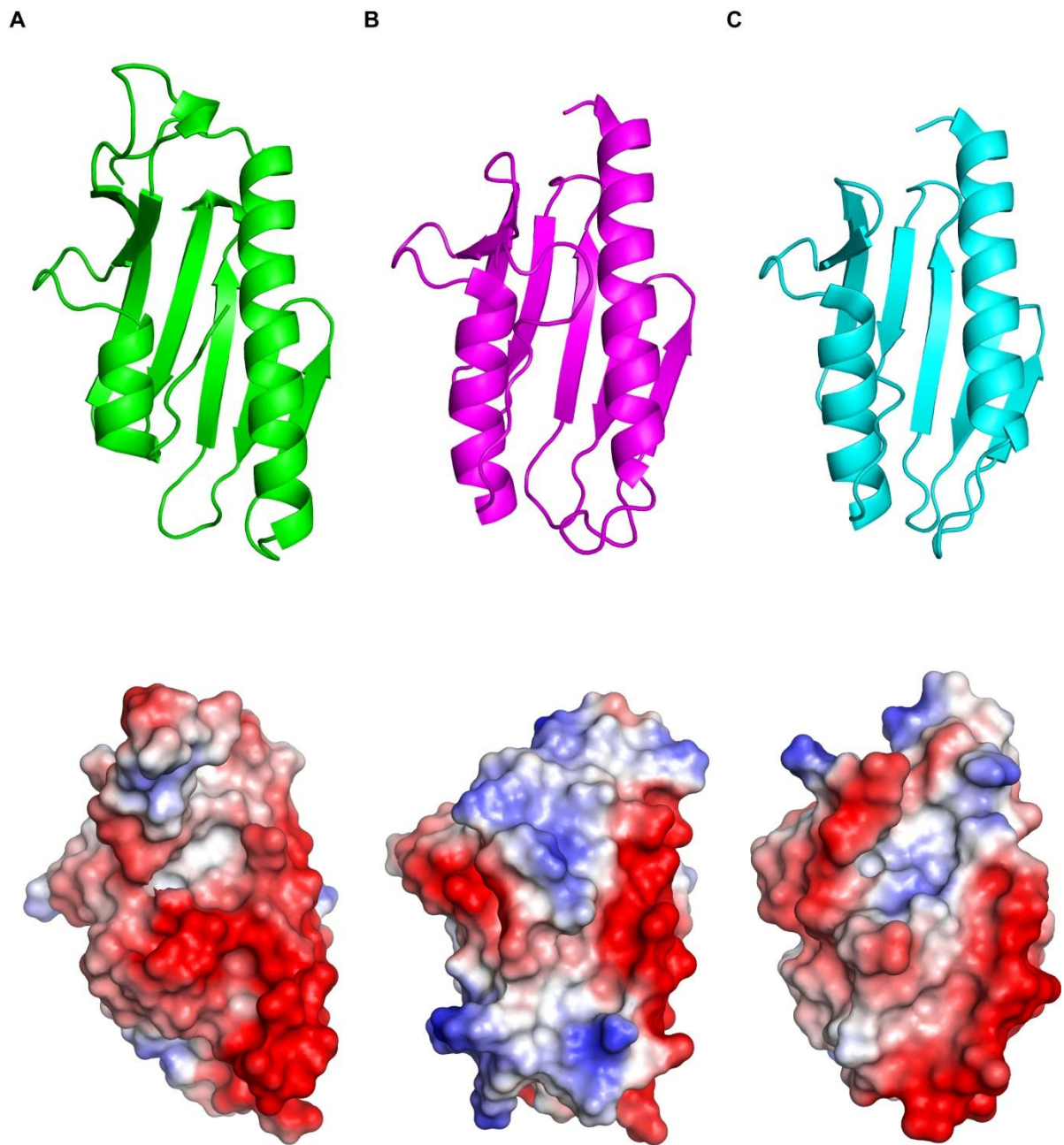
Figure 4 – Structural features of Ct-frataxin. Top: Comparison between the structures of Ct-frataxin. (A), human (3s4m) (B) and bacterial (1ew4) (C) frataxins. Bottom: electrostatic surfaces of frataxin in the same order as in the top.
