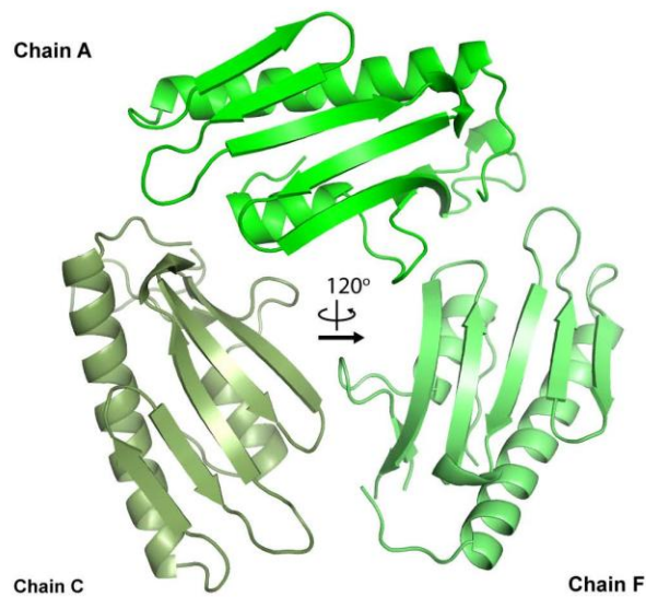
Figure 2 – Symmetry of the hexamer in the crystallographic unit. Top: The three possible crystallographic dimers. Bottom: Ternary symmetry between protomers. The different protomers are shown in different shades of green.
