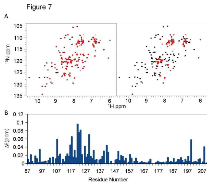
Figure 7 – Ct-frataxin is able to bind and inhibit the enzymatic function of bacterial IscS. A) Titration of labelled Ct-frataxin with unlabelled bacterial IscS at a 1:0.5 Ct-frataxin:IscS molar ratio (left) and at a 1:3 Ct-frataxin:IscS molar ratio (right). B) Chemical shift perturbation observed at low Ct-frataxin:IscS ratios plotted along the frataxin sequence.
