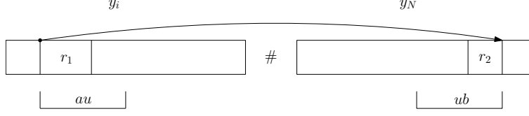
Figure 2: au starts where a word r_1 of R_{y_N}^\ell starts in y_i and ub ends where a word r_2 of R_{y_1\#...\#y_{N-1}}^\ell ends in y_N . Moreover, if |u| \geq \max\{|r_1|, |r_2|\} - 1 , then aub is a Case 2 MAW.
