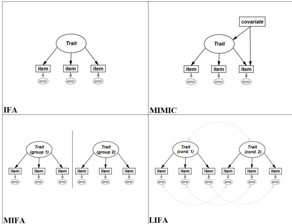
Figure 1: Model specifications (Trait: here IA or HI; Item: here symptom criterion; Error: residual variances; Group: here gender; Covariate: here age or co-occurring diagnoses; Cond. 1 and 2: here informants. Black arrows denote loadings and grey curved arrows denote correlations)
