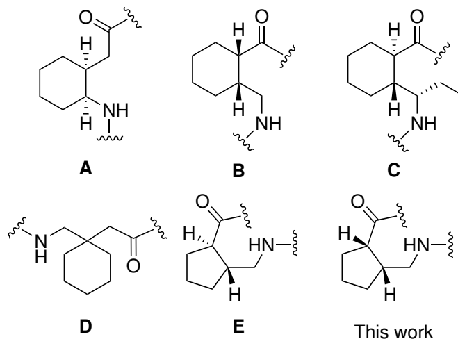
Figure 7: Constrained carbocyclic \gamma -amino acids that promote helical foldamers.
