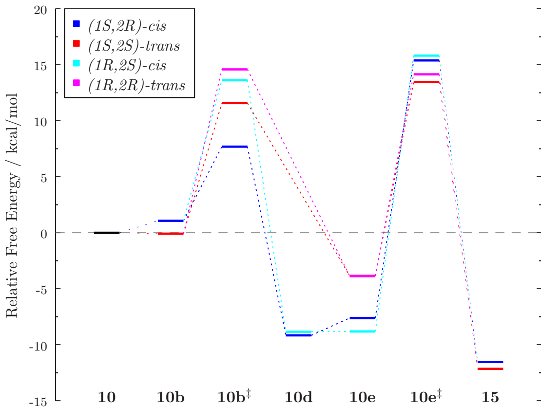
Figure 5: Calculated free energy profile of the investigated part of the mechanism depicted in scheme 2.
