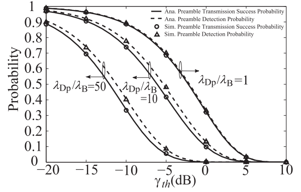
Fig. 3. The preamble detection probability \mathcal{P}_{\text{detection}}^1 and the preamble transmission success probability \mathcal{P}^1 versus the SINR threshold \gamma_{th} for the 1st single time slot. We set T^1 = 1 - e^{0.1} , \rho = -90 dBm, \sigma^2 = -90 dBm, \lambda_B = 10 BS/km 2 , \alpha = 4 , \gamma_{th} = -10 dB, and the baseline scheme is considered with \mathcal{R}^1 = 1 .
