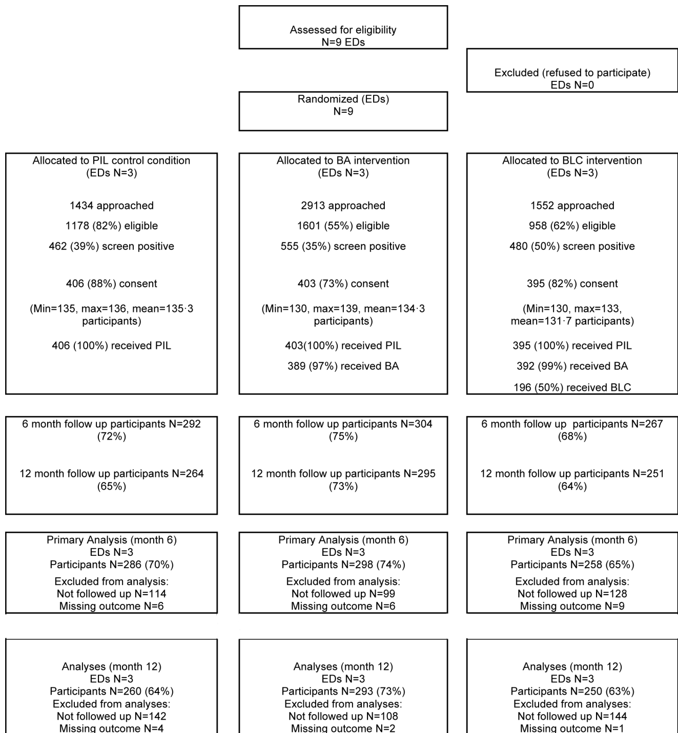
Figure 1. Consort Diagram.
