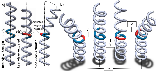
Fig. 2: Working principle of a single full turn of a SMA tendril as an independent 3-DOF joint. The SMA tendril is compressed when heated. a) Rear and side view of the tendril when one third (120 deg) of a full turn is activated (heated- in red). A twist along this section results a reduction in the helix pitch on the opposite side and hence bending the backbone in the opposite direction. b) Wiring diagram for different activation scenarios. V- power supply connection through a relay board and PWM current controller, G- permanent ground connection red- active (heated) section, blue- inactive (cold) section.
