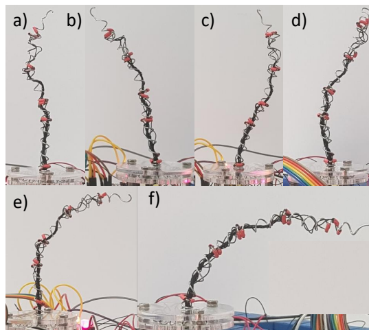
Fig. 1: Complex shapes resulted from actuating (local heating) different joints along an ATBR.
