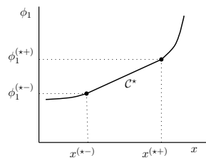
Fig. 3 A first-order transition showing as the linear section C^* in an isothermal section of the \phi_1 surface.
