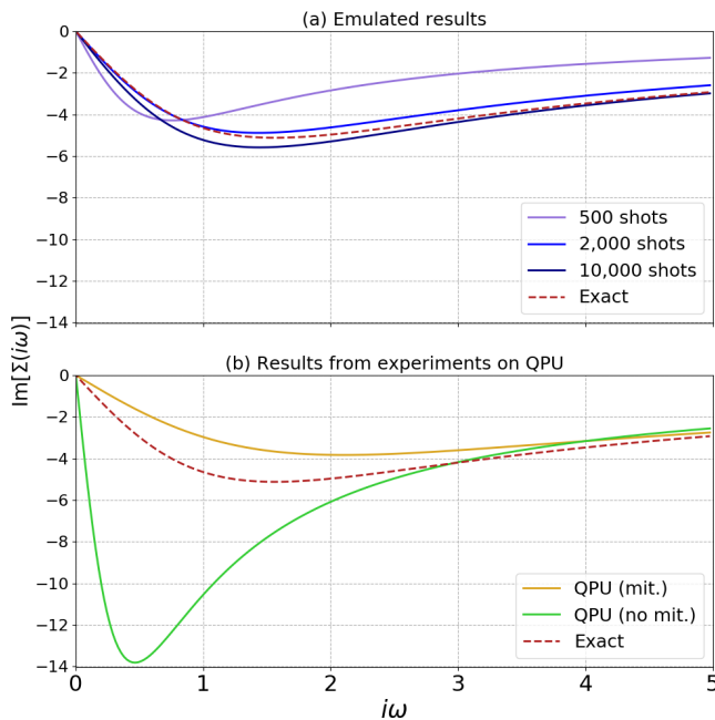
FIG. 6. Converged effective on-site Matsubara self-energy for the Bethe lattice Hubbard model with EwDMET at n_{\text{mom}} = 1 . (a) Upper plot shows results from the quantum simulator with finite sampling of the RDM elements, compared to exact results (infinite sampling). (b) Lower plot shows results from quantum hardware on IBMQ Santiago and IBMQ Bogota and 5,000 shots in the RDM sampling, with and without error mitigation in the RDM sampling respectively.
