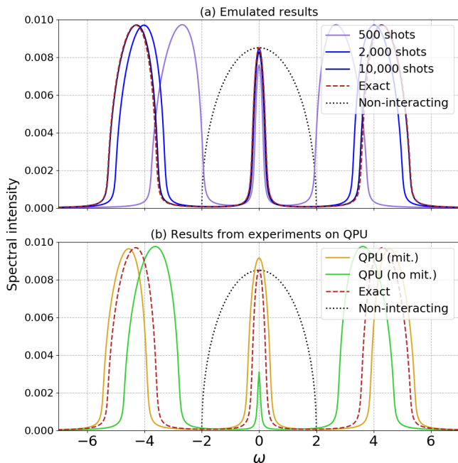
FIG. 5. The density of states for the Hubbard model on the Bethe lattice with infinite coordination for the EwDMET method with n_{\text{mom}} = 1 . (a) Upper results are performed on a classical QPU simulator with finite sampling noise and varying numbers of shots in the VQE solution to the cluster Hamiltonian at each iteration. (b) Lower panel shows results from two QPU experiments, on IBMQ Santiago and IBMQ Bogota, with and without error mitigation respectively, with 5,000 shots for the sampling of the required RDMs. Grey dotted lines show the original non-interacting spectrum of the model, while the red dotted line shows the EwDMET( n_{\text{mom}} = 1 ) results with an exact solution of the cluster Hamiltonian each iteration.
