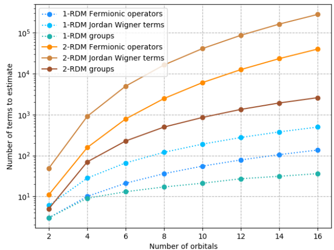
FIG. 7. Number of unique fermionic operators, corresponding set of unique Pauli strings (under Jordan-Wigner mapping), and commutative groups to be measured in order to compute all elements of the one-body (dotted line) and two-body RDM (solid line), for up to 16 orbitals (32 qubits). The groups were found via the Largest-degree First Coloring (LDFC) algorithm.
