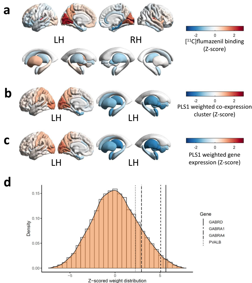
Fig. 3 [ 11 C]flumazenil binding follows a postero-anterior gradient and spatially tracks PVALB , GABRD , GABRA1 and GABRA4 expression. Z-scored regional brain distribution of a [ 11 C]flumazenil binding, b weights of covariance between [ 11 C]flumazenil signal and 52 co-expression clusters from the AHBA and c weights of covariance between [ 11 C]flumazenil signal and expression of genes from the AHBA. d Density plot of Z-scored weight distribution of genes from the AHBA in their covariance with [ 11 C]flumazenil signal, with location of GABRD , GABRA1 , GABRA4 and PVALB . GABRA1 , GABA A receptor subunit α1, GABRA4 , GABA A receptor subunit α4, GABRD , GABA A receptor subunit δ, PVALB , parvalbumin.
