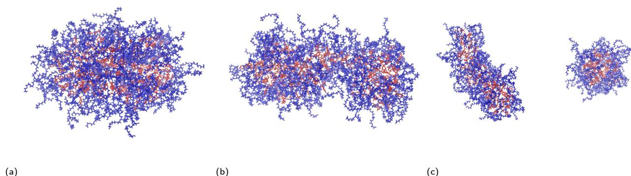
Fig. 9 Snapshots of the indomethacin-loaded TX-100 micelle at (a) t = 100 ns, (b) t = 300 ns and (c) t = 600 ns. As shown in these snapshots, the TX-100 micelle splits into two daughter micelles of different sizes after 300 ns during the indomethacin solubilisation process. Red and blue show the tails and the headgroups of surfactants respectively.
