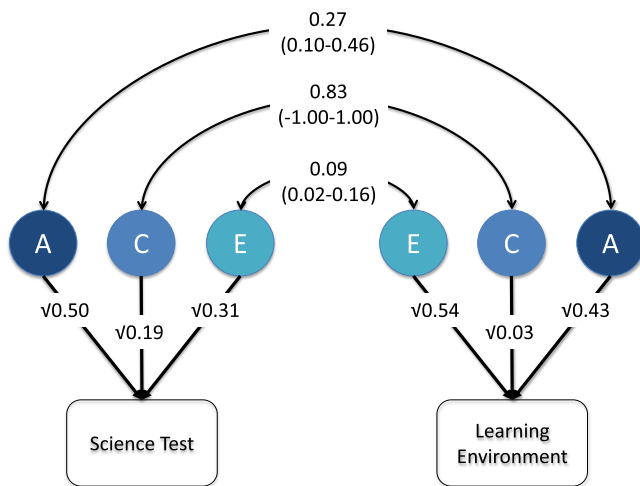
Fig. 1. Bivariate model between test and environment. Note. A = additive genetic; C = shared environment; E = non-shared environment; 95% confidence intervals in parentheses for the genetic and environmental correlations between the test and environment. 95% confidence intervals for the ACE estimates can be found in Table 4. The 95% confidence interval for the shared environment correlation is very large because of the small variance attributed to shared environmental influence, especially on the learning environment measure. We had the option of dropping the non-significant shared environmental component for the learning environment measure. We decided not to do this because the full ACE model provides the most accurate point estimates for all of the parameters. Dropping the shared environment for the learning environment measure would have meant also dropping the shared environmental overlap between the learning environment and science performance, and we felt that it was important to include all of the environmental parameters in the analysis of the overlap between an environmental variable (the science learning environment) and the outcome (science performance). Finally, the genetic and environmental correlations must be interpreted with caution because of the low phenotypic correlation of 0.225 between these two measures.
