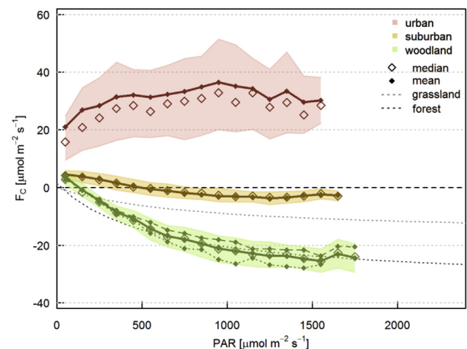
Fig. 7. Relation between carbon dioxide fluxes and photosynthetically active radiation (PAR) for summer daytimes (June–August 2011 and 2012), i.e. when leaves are fully out. PAR data are used to group the fluxes into bins of 100 \mu\text{mol m}^{-2} \text{ s}^{-1} , with only those bins containing >25 data points shown. The interquartile range for each site is shaded. Dashed lines are empirical models for temperate grassland (Flanagan et al., 2002) and broadleaf forest (Schmid et al., 2000). For the woodland site, the relations for 2011 (dashed line) and 2012 (dotted line) are also shown separately.
