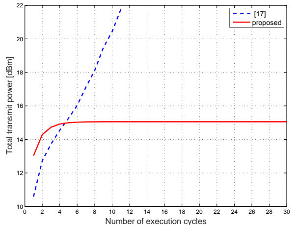
Fig. 4. Convergence comparison between the proposed approach and the single-cell scheme described in [17] with \rho = 0.3 , \sigma^2 = 0.1 and SINR=14dB.
