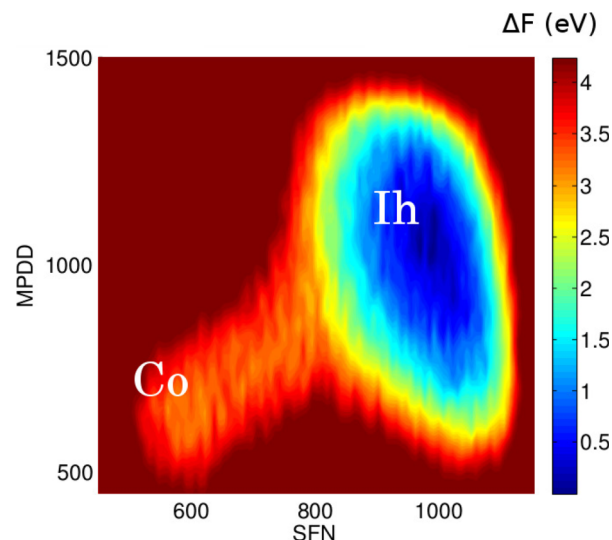
FIG. 10. Co and Ih basin free energy surface reconstruction for a \text{Ag}_{92}^{\text{shell}}\text{Pt}_{55}^{\text{core}} . Hot colours in the CV space highlight a high free energy of the corresponding configuration.
