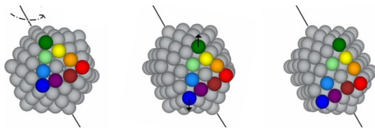
FIG. 5. Initial, saddle, and final configurations of DSD mechanism for Ih into Dh transformation. Multicolored atoms delimit a facet in the original Ih. Rotation along the depicted axis is of 36^\circ .
