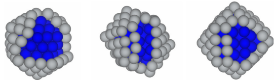
FIG. 8. Initial, saddle, and final configurations in the case of Dh into Ih transformation in \text{Ag}_{shell}^{92}\text{Pt}_{55}^{core} . Ag atoms are in grey, Pt in blue. Few atoms from Ag shell are removed to show Pt inner core.
