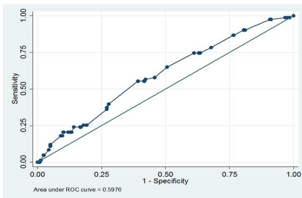
Figure 3: ROC curve for in-hospital mortality for Thoracoscopic using NLCA data 2010- 2012
