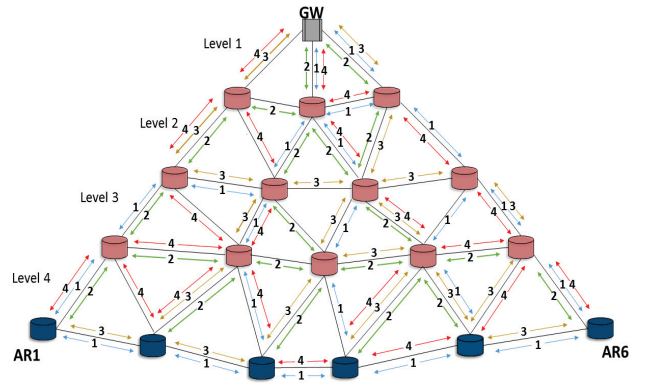
Fig. 1: Sub-topology (T1M5, see TABLE I) of the 19 node based network. 4 RPs are demonstrated.
