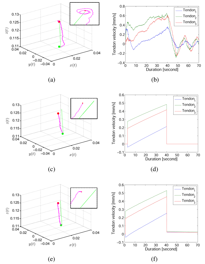
Fig. 12. Experimental results of a trajectory tracking execution via fuzzy-model-based approach (shown by (a) and (b)), open-loop Jacobian based approach (shown by (c) and (d)), and closed-loop Jacobian based approach (shown by (e) and (f)). The figures in left column show the experimental recorded trajectory in 3D space and the zoom-in view around the target. The green dot indicates the initial position and red dots indicate the termination positions. The green line shows the specified reference trajectory. The magenta trajectory indicates the trajectory based on the applied controller. The figures in right column show the tendon speed control signals.
