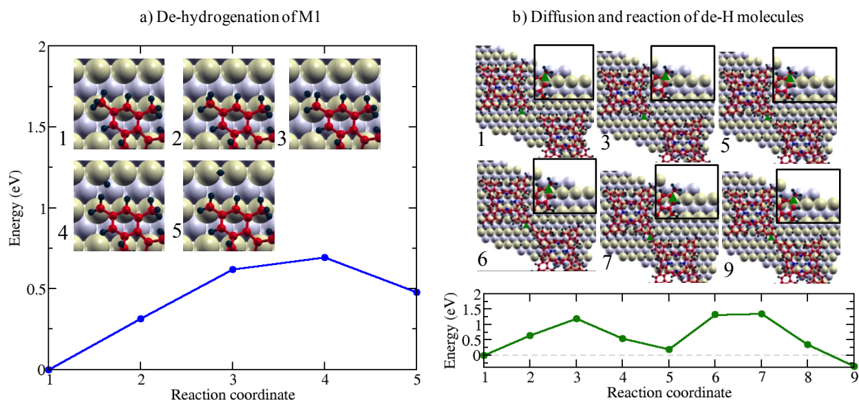
Figure 8. Modeling the “independent” scenario: Minimum energy profile and reaction path bringing two fully hydrogenated molecules, M1 and M2, placed initially far apart on the surface (as in Fig. SI-9a), to the bonded configuration as in Fig. 6(b) via the mechanism whereby the two dehydrogenations, diffusion and bonding happen independently one after another as described in the text. (a) Dehydrogenation reaction involving a 4-methyl hydrogen atom. The initial state (reaction coordinate R_c=1 ) is the stable configuration of the intact, fully hydrogenated molecule (reference energy 0 eV). In the final state at R_c=5 , M1 is dehydrogenated, with the removed hydrogen atom placed nearby on the free surface. The reaction path shows how the H atom avoids passing through a higher energy barrier in the central hollow position between 4 top-most Cu atoms. Note that \Delta E_{rem} is the difference between the final and initial states. The minimum energy profile for dehydrogenation of M2 is the same. (b) Minimum energy profile and reaction path corresponding to the diffusion of M1 along the Cu rows towards M2 followed by the diagonal bonding between two 4-methyl groups of both molecules. The insets highlight the bonding region. At R_c=1 the molecules are non-bonded and dehydrogenated. The peak at R_c=3 stems from the bond breaking with the surface during the M1 diffusion along the row, which at the minimum ( R_c=5 ) reaches the next equilibrium position. After a further diffusion and initial interaction with M2 ( R_c=6,7 ), the two molecules eventually connect ( R_c=7-9 ). The energy gain of the final bonded configuration at R_c=9 relative to the initial state ( R_c=1 ) of 0.58 eV indicates that two previously dehydrogenated molecules are driven to connect.
