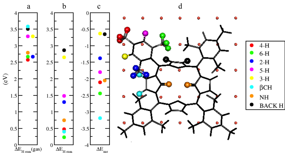
Figure 4. Removal energies of H atoms from non-equivalent positions in TMTPP: (a) in the gas-phase, \Delta E_{rem}(gas) , and (b) adsorbed on Cu(110), \Delta E_{rem} ; (c) the influence of the surface in each dehydrogenation process is quantified by \Delta E_{sur} = \Delta E_{rem} - \Delta E_{rem}(gas) . The different types of H atoms are shown in (d) in the molecular structure by the corresponding color code. The removal energies shown are equivalent to dissociation energies; note, the final position of the removed H atoms is on the surface next to the molecule. Although energy barriers for the dehydrogenation reaction provide a better indicator of the ability to dehydrogenate, a systematic calculation of the energy barriers for all non-equivalent H atoms was performed only for the hydrogen atoms from the 4-methyl groups (see Fig. 6a). However, it is obvious that the barriers cannot be smaller than the energy difference \Delta E_{rem} between the initial and final states, hence \Delta E_{rem} serves as a realistic guide of the ease with which H atoms can be removed from various positions in the molecule. Note that H atoms belonging to a specific methyl group are inequivalent on the surface. However, their removal energies were found to be the same, since the rotational flexibility of the group enables it to relax to the same final configuration.
