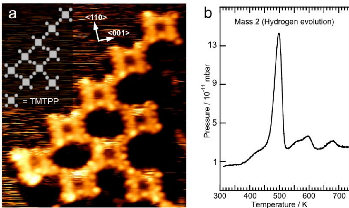
Figure 3. a) An experimental STM image of a covalently bonded network of TMTTPP molecules following heating to 600 K, ( 65 \times 73 \text{ \AA}^2 , 0.236 V, 0.35 nA). The inset shows a pictorial representation of the networked structure imaged. b) Temperature Programmed Desorption data showing the evolution of \text{H}_2 during the coupling process. STM images of larger areas are given in the SI (Fig. SI-12).
