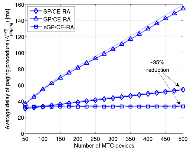
Fig. 6. Average delay of paging procedures with CE-RA.
