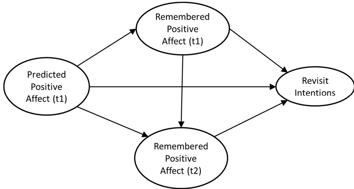
Figure 1: Research Model
