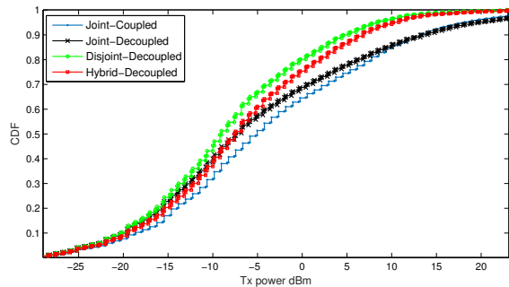
Fig. 5. CDF of the devices' transmit power.
