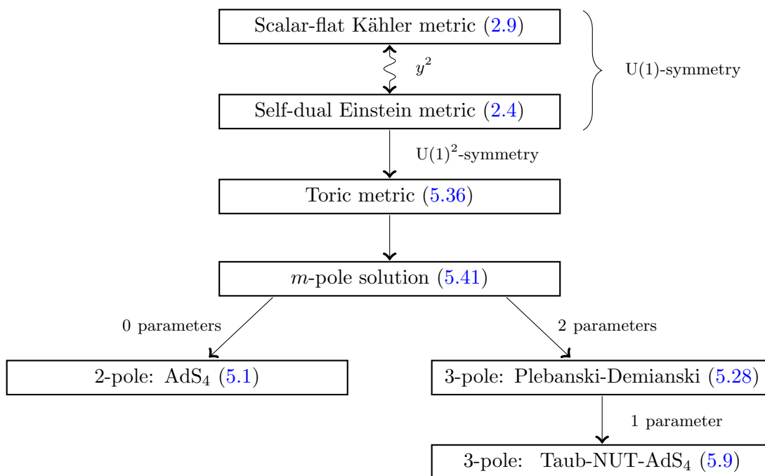
Figure 1. Overview of the metrics discussed in the main part of the paper and in the present appendix. The arrows point from a metric to a special case of the metric, except the wavy arrow which corresponds to a conformal transformation, i.e. equation (2.9).
