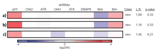
Fig. 5 RNAi signatures derived from the treatment of Eμ-Mycp 19arf -/- lymphoma cells with a) 3c , b) dichloro(1,10-phenanthroline)copper(II), and c) the necroptosis-inducing rhenium(V)-oxo complex at the LD 80-90 concentration for each compound.
