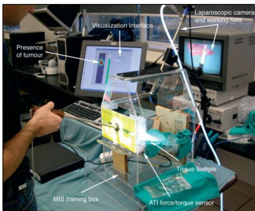
Fig. 3 The Tactile Sensing System (TSS) [55].
