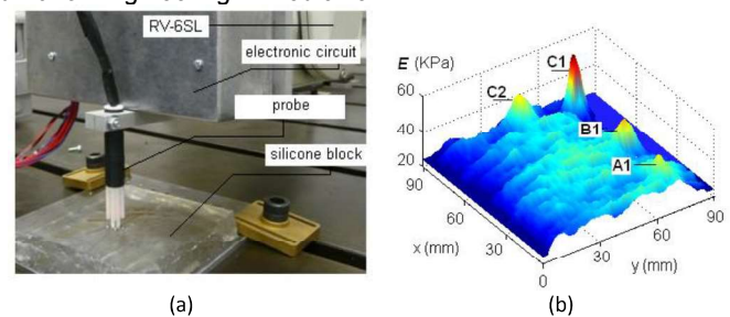
Fig. 2 The rolling indentation experiment setup shown in (a) and the stiffness map produced by the rolling indentation probe shown in (b) [11].
