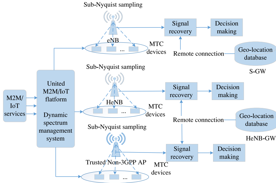
Fig. 5. Proposed hybrid framework combining compressive spectrum sensing and geolocation database in M2M networks.
