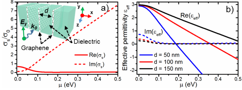
Fig. 1. (a) Graphene complex conductivity normalized to \sigma_0 = e^2/4h = 0.061 mS for T = 300 K, \gamma = 10^{-12} s ^{-1} at f = 20 THz. (Inset) Geometry of the graphene-dielectric metamaterial. (b) Complex effective permittivity, \epsilon_{eff} , for \epsilon_m = 3 , T = 300 K, f = 20 THz and different values of spacer thickness d . Solid and dashed lines stand for real and imaginary parts, respectively.
