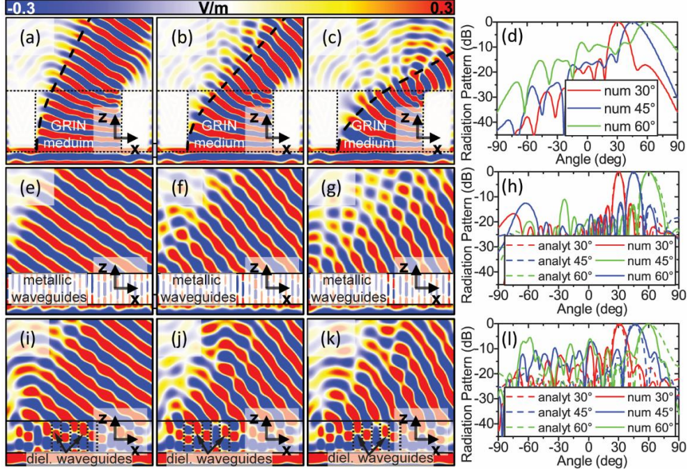
Fig. 3. Numerically calculated magnitude of the E_y -field for the first (a-c), second (e-g) and third design (i-k) for output angles: \theta = 30^\circ (first column, a,e,i), \theta = 45^\circ (second column, b,f,j), \theta = 60^\circ (third column, c,g,k). Black dashed lines in (a-c) represent the analytical solutions for the ray propagation inside the GRIN medium. (d), (h) and (l) show the radiation patterns of the BS1, BS2, and BS3, respectively, analytically (dashed) and numerically (solid) calculated for the output angles of 30^\circ (red), 45^\circ (blue), and 60^\circ (green).
