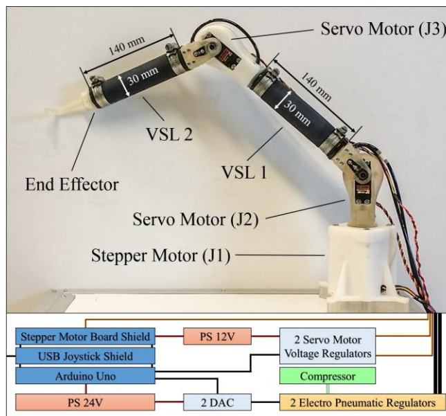
Figure 1 – Conceptual architecture of the anthropomorphic manipulator developed to assess the performance of the VSL.
