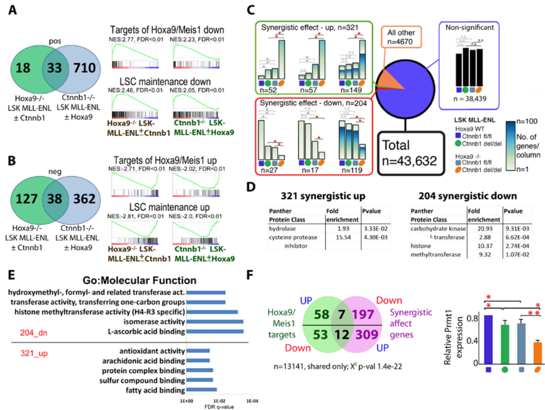
Figure 5. \beta -catenin and Hoxa9 co-regulate Prmt1 in LSK-MLL-ENL cells. (A, B) Venn diagram showing the overlap of 33 commonly enriched upregulated (A) and 38 commonly enriched downregulated (B) highly significant (FDR<0.05) gene sets between indicated comparisons (i.e., \beta -catenin inactivation in Hoxa9 -/- LSK-MLL-ENL, Hoxa9 inactivation in Ctnnb1 -/- LSK-MLL-ENL cells), including “Hoxa9/Meis1_DN” (Hess et al., 2006), “LSC_maintenance_down” (Somervaille et al., 2009), “Hoxa9/Meis1_UP” (Hess et al., 2006) and “LSC_maintenance_up” (Somervaille et al., 2009) as indicated. (C) A small set of genes is synergistically regulated by \beta -catenin and Hoxa9 (the effect of knockout of both genes is smaller or larger than could have been predicted from their single knockouts). Example sets of genes synergistic up-regulated (top), down-regulated (bottom) and non-significantly regulated (bottom right) are shown (all sets are in Figure S5). Keys and colour code in the top corner indicate the origin and the \beta -catenin and Hoxa9 status of MLL-ENL transduced cells. (D) Pantherdb protein classes ( http://pantherdb.org/ ) are shown for the 321_synergistic_up and 204_synergistic_down genes as indicated. P-value was obtained after Bonferroni correction. (E) The FDR q-values of the top5 Toppgene GO:Molecular function ( https://toppgene.cchmc.org/enrichment.jsp ) are shown for the synergistic up and downregulated genes as indicated. (F) Statistically significant directionality in the overlap of the synergistic genes with the Hox/Meis1_DN gene set (Dataset EV5B) including Prmt1, which has also been independently validated by RT-qPCR (right panel). See also Appendix figure S5.
