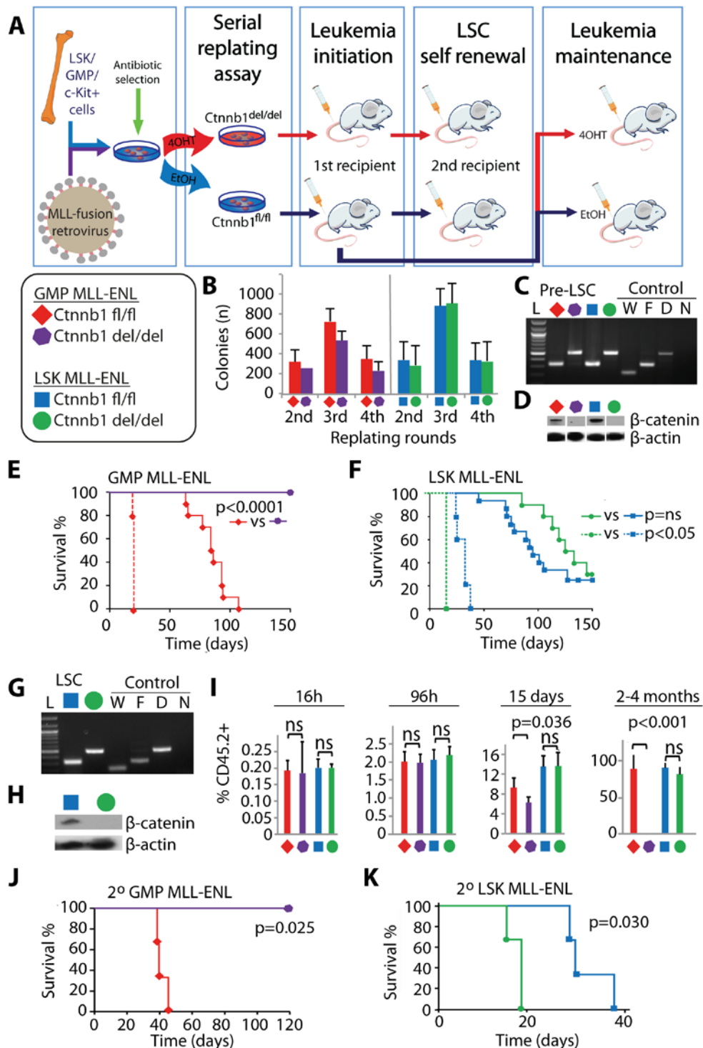
Figure 1. MLL-ENL leukemic stem cells derived from LSK or GMP populations have contrasting functional requirements of \beta -catenin for their initiation and maintenance of disease. (A) Schematic overview of the experimental procedures. Keys and colour codes in the legend box indicate the cells-of-origin and the \beta -catenin status of MLL-ENL transduced cells in the following experiments (B-K). (B) Colony numbers in serial replating assay of the different MLL-ENL transduced cells. Data are represented as mean \pm SD (C, G) PCR validation of Ctnnb1 deletion on genomic DNA isolated from the indicated MLL-ENL transduced GMP and LSK cells (C) or leukemic cells (G). L, 100bp ladder; W, wild type control, F, Ctnnb1 floxed allele, D,
