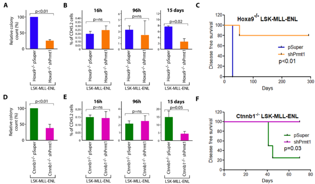
Figure 7. Suppression of Prmt1 abolishes \beta -catenin or Hoxa9 independent transformation in HSC-derived MLL-CSCs. (A) The relative number of colonies from Hoxa9 -/- LSK-MLL-ENL leukemic cells with empty vector or shPRMT1. Data are represented as mean \pm SD. (B) The % of CD45.2+ donor cells in the bone marrow of recipient mice at the indicated time points post-transplantation of Hoxa9 -/- LSK-MLL-ENL leukemic cells with empty vector or shPrmt1. Data are represented as mean \pm SD. (C). Kaplan-Meier survival curve of secondary recipient mice transplanted with Hoxa9 -/- LSK-MLL-ENL leukemic cells with vector control or shPrmt1. (D) The relative number of colonies from Cttnb1 -/- LSK-MLL-ENL leukemic cells with empty vector or shPRMT1. Data are represented as mean \pm SD. (E) The % of CD45.2+ donor cells in the bone marrow of recipient mice at the indicated time points post-transplantation of Cttnb1 -/- LSK-MLL-ENL leukemic cells with empty vector or shPrmt1. Data are represented as mean \pm SD. (F). Kaplan-Meier survival curve of secondary recipient mice transplanted with Cttnb1 -/- LSK-MLL-ENL leukemic cells with vector control or shPrmt1. See also Appendix figure S6.
