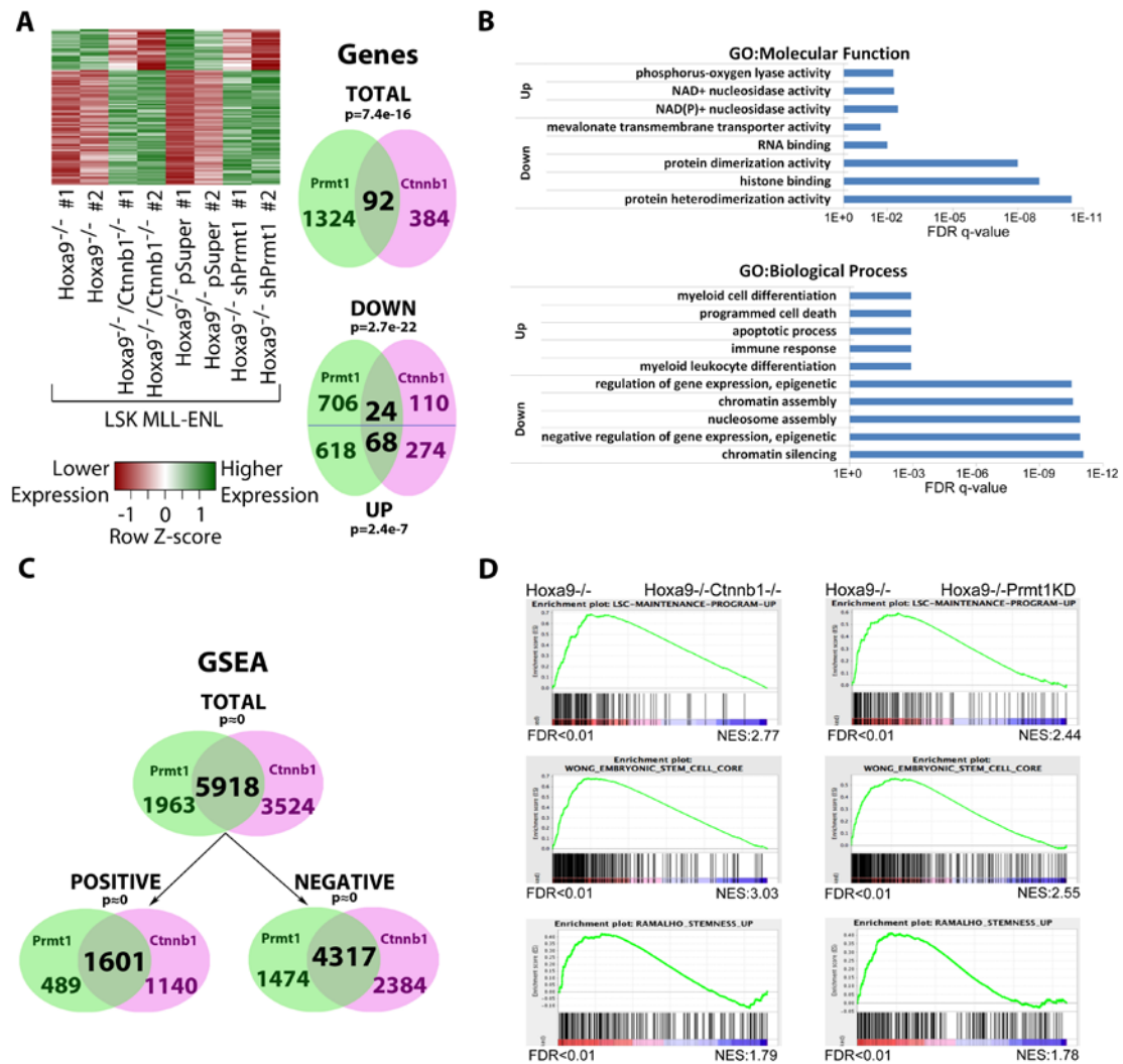
Figure 6: Prmt1 regulates similar and overlapping transcriptional programs mediated by \beta -catenin in LSK-MLL-ENL cells. (A) Heatmap analysis and Venn diagram showing the commonly regulated genes after the loss of function of Prmt1 and \beta -catenin in Hoxa9 -/- LSK-MLL-ENL cells. (B) The FDR q-values of the top GO:Molecular function (top panel) and GO:Biological process (bottom panel) ( https://toppgene.cchmc.org/enrichment.jsp ) for the indicated up- and down-regulated genes is shown. (C) Venn diagrams showing the total, positively and negatively regulated genesets identified by GSEA upon the loss of function of Prmt1 and \beta -catenin in Hoxa9 -/- LSK-MLL-ENL cells. (D) Examples of stem cell and stemness signatures which were commonly higher expressed in the single knockout Hoxa9 -/- LSK-MLL-ENL cells compared to Prmt1 down-regulated or \beta -catenin inactivated Hoxa9 -/- LSK-MLL-ENL cells.
