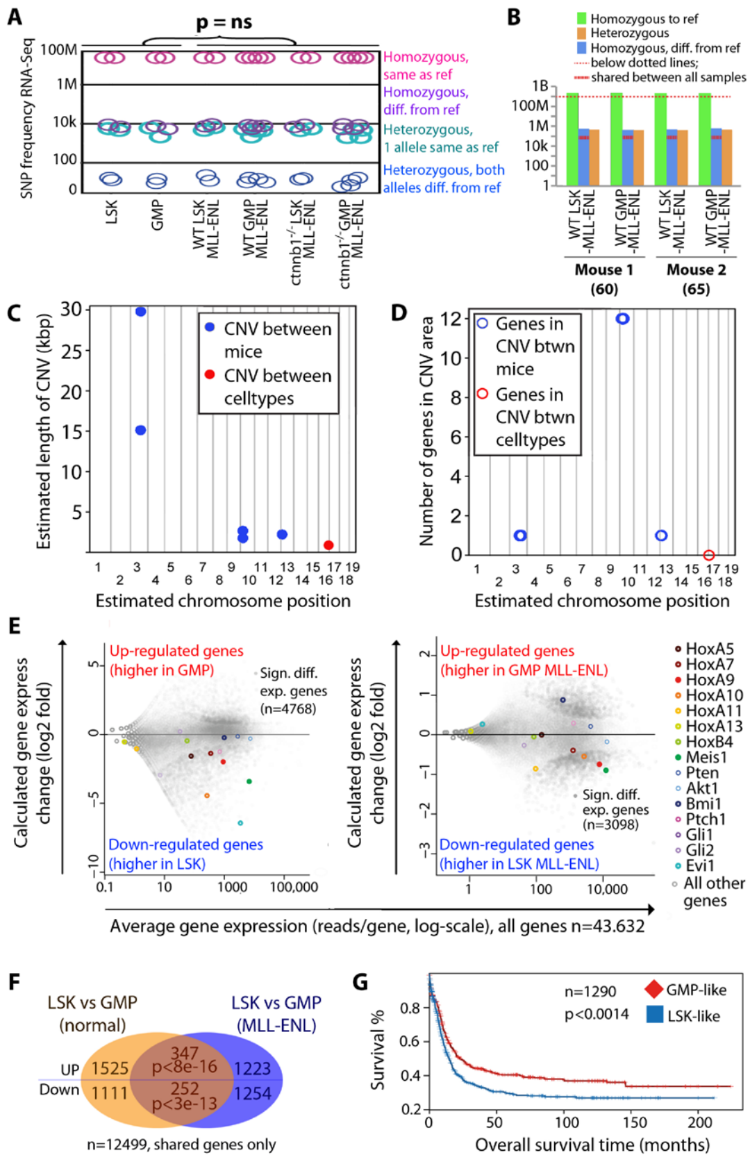
Figure 2. Cells-of-origin transcriptional-memory predicts survival in AML patients. (A-B) Number of identified genomic variants in indicated MLL-ENL transformed cells using RNA-Seq (A) and genomic sequencing (B). A two-tailed t-test was performed in (A). LSK, wildtype LSK cells; GMP, wildtype GMP cells. (C, D) Manhattan plots indicating estimated length of CNVs (C) or number of genes in
