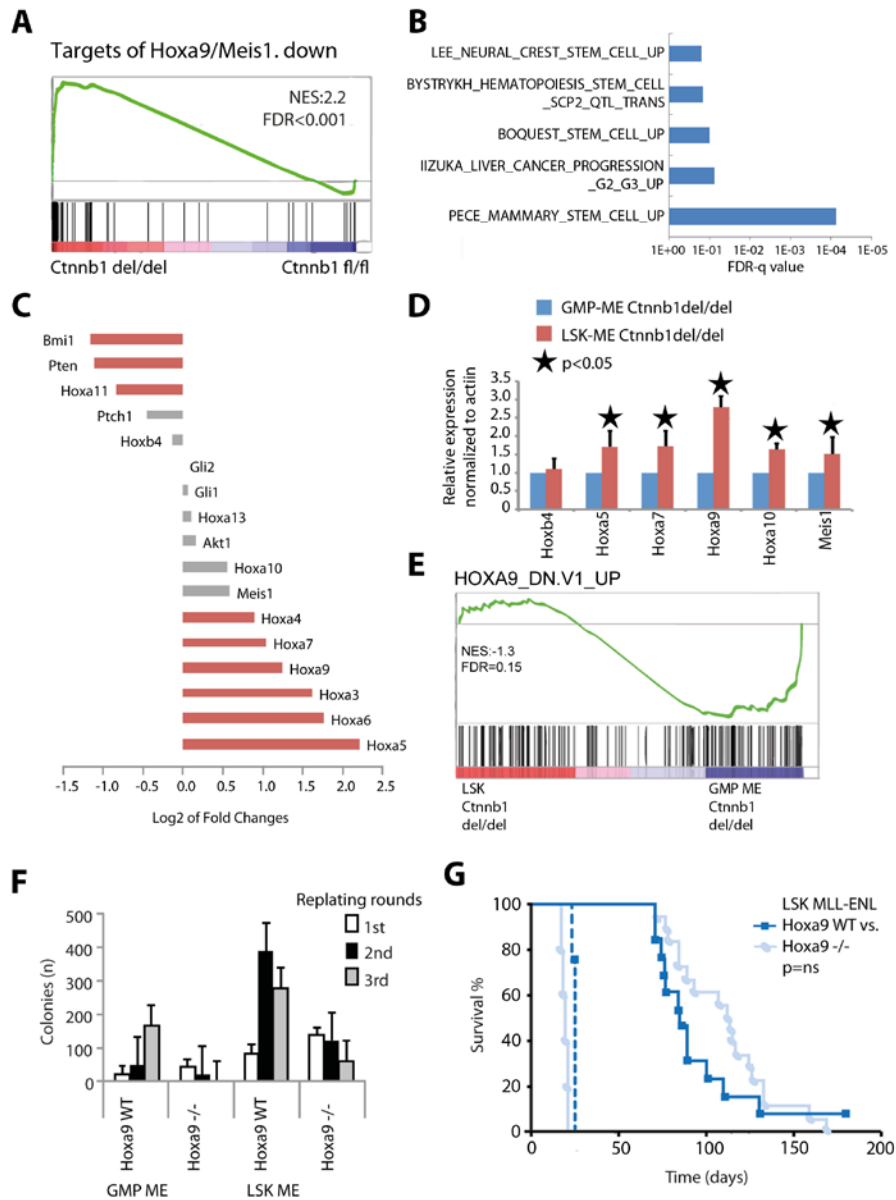
Figure 3. Key transcriptional-memory gene Hoxa9 may help to overcome \beta -catenin dependent transformation in LSK-derived MLL-CSCs. (A) Gene set enrichment analysis (GSEA) shows “Targets of Hoxa9/Meis1 , down” (Hess et al., 2006) for the indicated comparison. (B) Log 10 -fold FDR q-values of the indicated gene sets positively enriched in \beta -catenin deleted LSK-MLL-ENL compared to \beta -catenin deleted GMP-MLL-ENL. (C-E) RNA-seq log 2 -fold change of key self-renewal genes (C), RT-qPCR validation of Hox/Meis1 expression represented as mean \pm SD of 3 independent experiments. Two-tailed t-test was performed (D), and GSEA showing “ Hoxa9 _dn.v1_up” (Faber, Krivtsov et al., 2009) for the \beta -catenin deleted LSK-MLL-ENL to \beta -catenin deleted GMP-MLL-ENL comparison (E). (F) Colony numbers in serial replating assay of indicated MLL-ENL transduced cells. Data are represented as mean \pm SD. (G) Kaplan-Meier survival curve of mice transplanted with Hoxa9 -/- (n=18) or WT LSK-MLL-ENL (n=13) transformed cells (solid lines) and secondary recipient mice (n=5 for Hoxa9 -/- and n=4 for wt, dotted lines) as indicated. Comparisons between Hoxa9 WT and Hoxa9 -/- were not significantly different (ns). See also Appendix figure S3.
