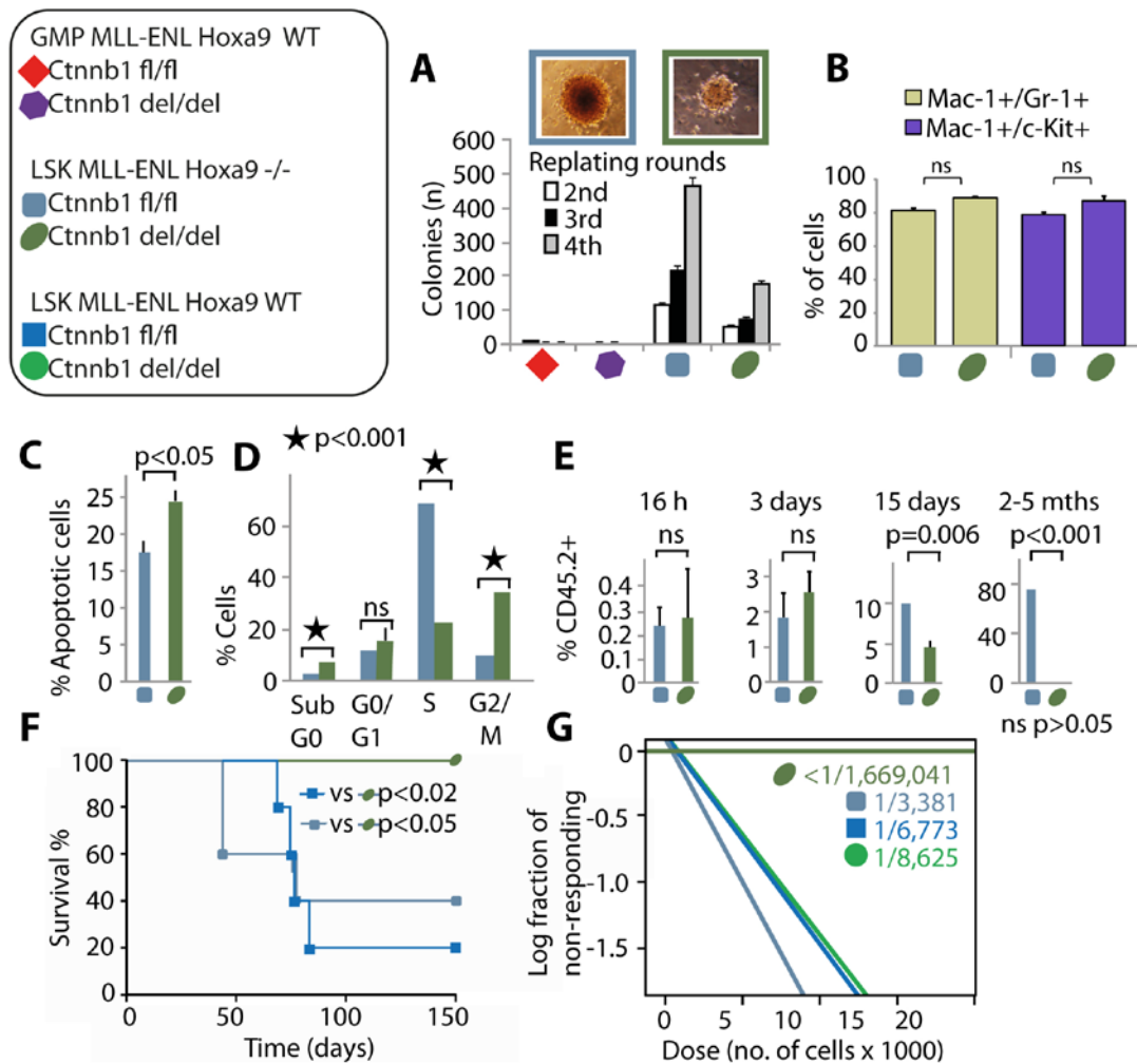
Figure 4. Deletion of both \beta -catenin and Hoxa9 abrogates leukemia development in LSK-MLL-ENL cells. Keys and colour code in the left top corner indicate the origin and the \beta -catenin and Hoxa9 status of MLL-ENL transduced cells. (A) Colony numbers in serial replating assay of MLL-ENL transduced cells. Images of typical 4 th round colonies shown above. Data are represented as mean \pm SD. (B) Summary of immunophenotypic analysis (Figure S4D) of LSK-MLL-ENL Hoxa9 -/- Ctnnb1 fl/fl with or without 72h Tamoxifen treatment. Data are represented as mean \pm SD. N=3, two-tailed t-test was performed. (C-E) % of apoptotic cells (AnnexinV assay) (E), cells in the indicated cell cycle phases (BrdU assay) (F) and CD45.2+ donor cells in the bone marrow of recipient mice at the indicated time points post-transplantation (G) of LSK-MLL-ENL transduced cells. Data are represented as mean \pm SD. N=4, two-tailed t-test was performed. (F) Kaplan-Meier survival curve of mice transplanted with LSK-MLL-ENL carrying different Hoxa9 and Ctnnb1 genotypes. N=5 per genotype was used. (G) Summary of the LSC frequencies obtained from the in vivo limiting dilution experiments (Figure S4E-H) using the LSK-MLL-ENL leukemic cells with different genotypes. See also Appendix figure S4.
