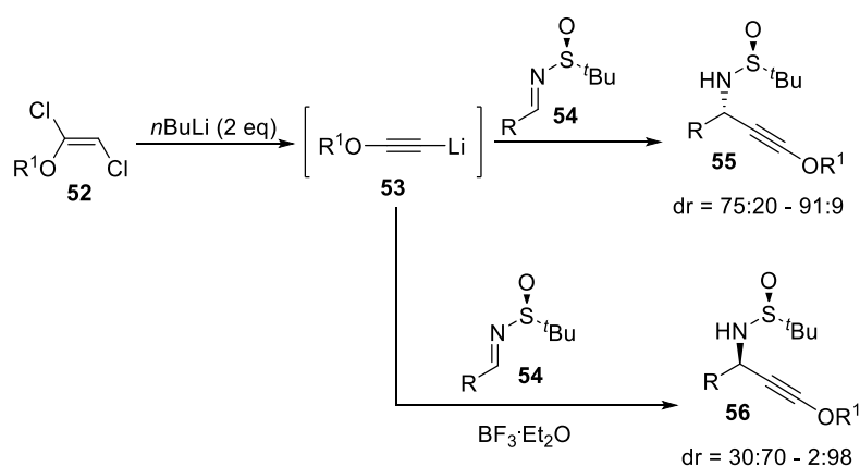
Scheme 13. Addition of lithiated ynol ethers to chiral N -sulfinyl imines.
