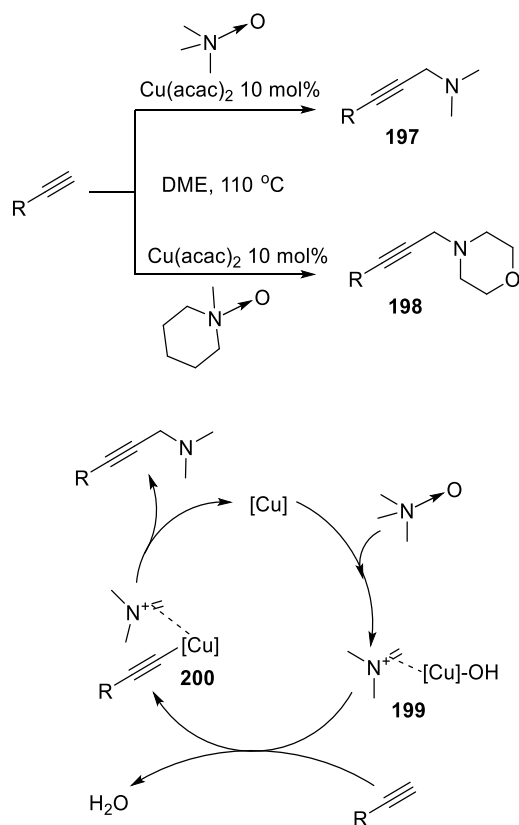
Scheme 41. Cu(II)-catalyzed oxidative alkynylation reaction of trialkylamine N -oxides.
