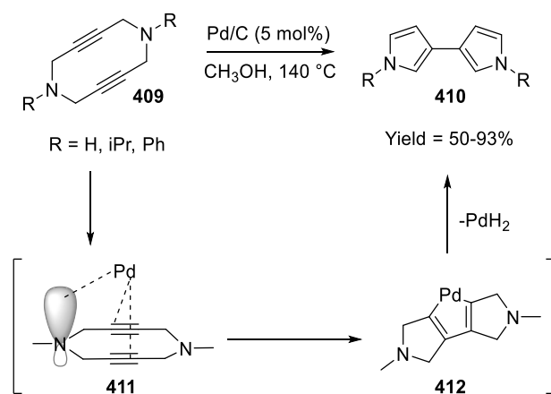
Scheme 91. Synthesis of bispyrrole 410.
