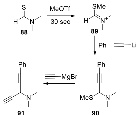
Scheme 20. Addition of lithium acetylides and Grignard reagents to thioiminium salts.
