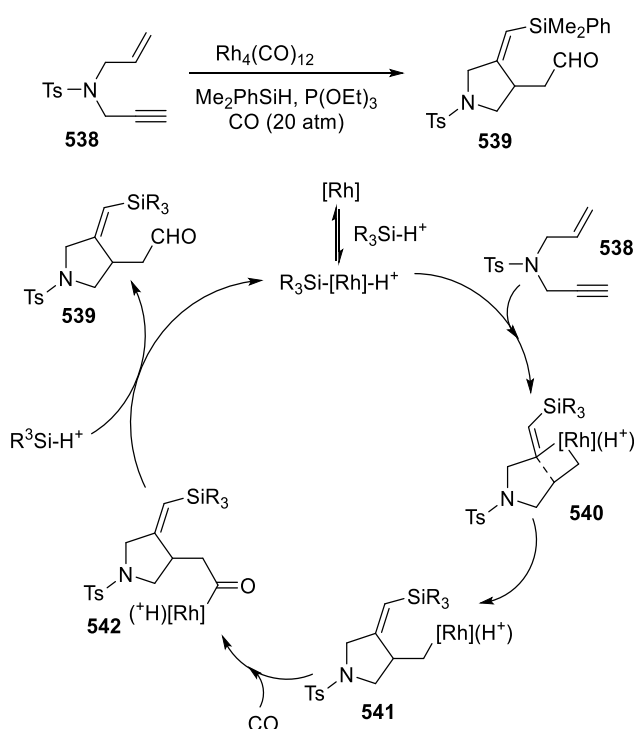
Scheme 112. Rhodium catalyzed carbonylative silylcarbocyclization reaction of enynes.
