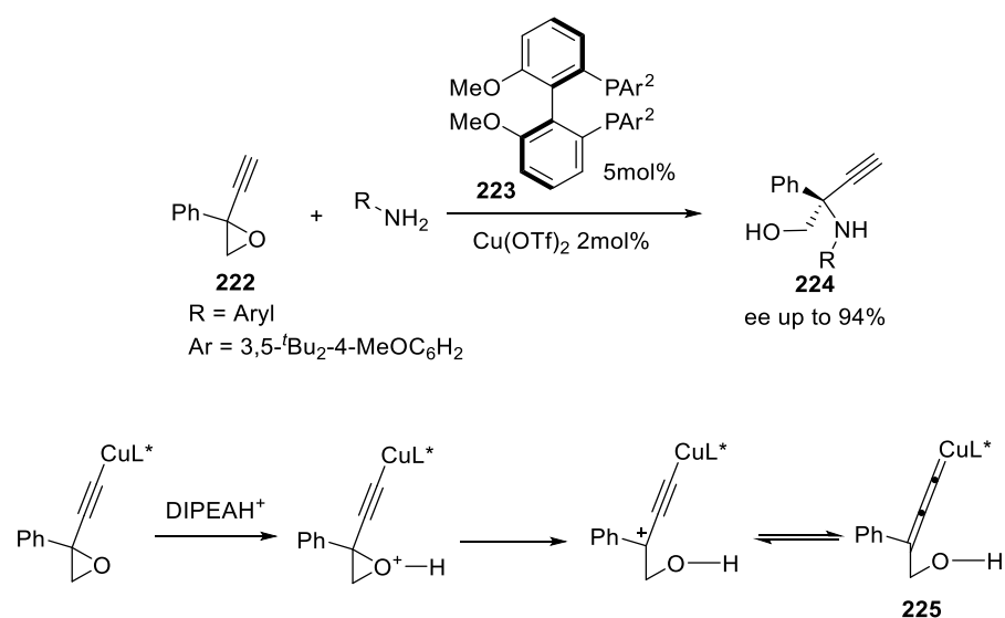
Scheme 46. Synthesis of tertiary propargylamines 224 from epoxide 222.
