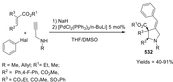
Scheme 110. Synthesis of pyrrolidines 532.
