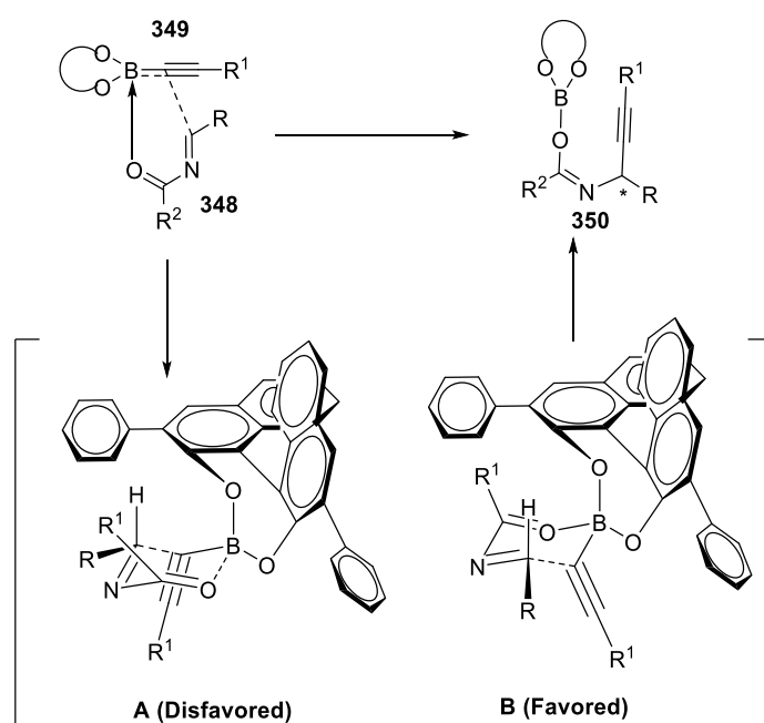
Scheme 78. Transition state in the alkylation of N -acylimines with alkynylboronates.
