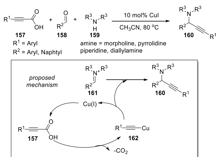
Scheme 33. Synthesis of propargylamines from alkynyl carboxylic acids.
