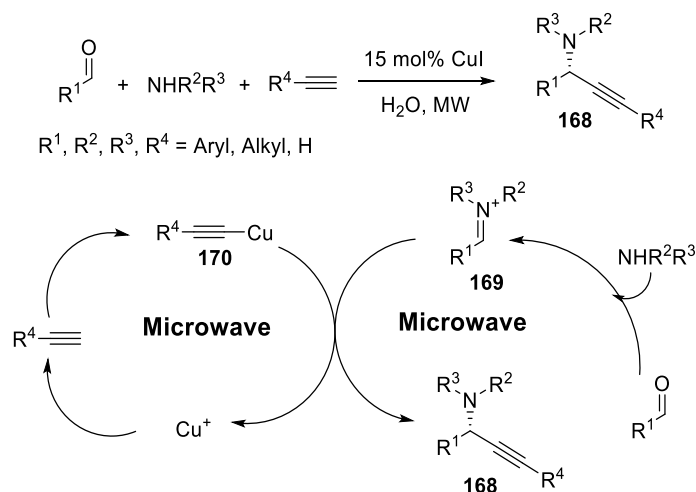
Scheme 35. Microwave assisted copper catalyzed synthesis of propargylamines 236.
