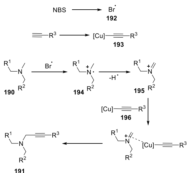
Scheme 40. Alkynylation of tertiary amines with CuBr/NBS catalytic system.
