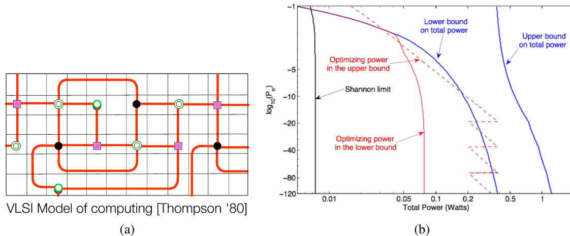
Fig. 14. (a) Thompson's VLSI model of computing. (b) Energy with a model of computation that only considers energy consumed in computational nodes.
