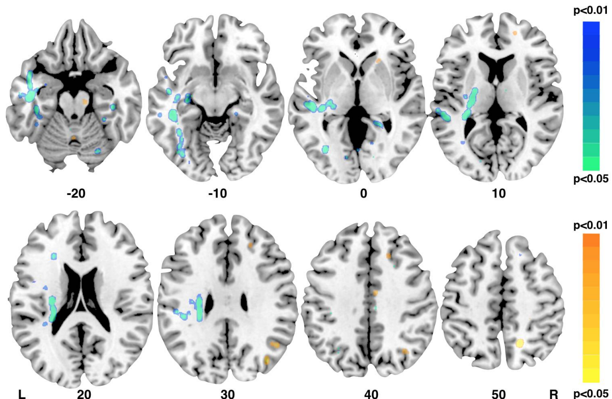
Figure 5 Tract-based spatial statistics (TBSS) analysis of acute imaging fractional anisotropy (FA) values and longitudinal language recovery (follow-up AQ). Cold colours indicate FA voxels negatively associated with longitudinal symptom
