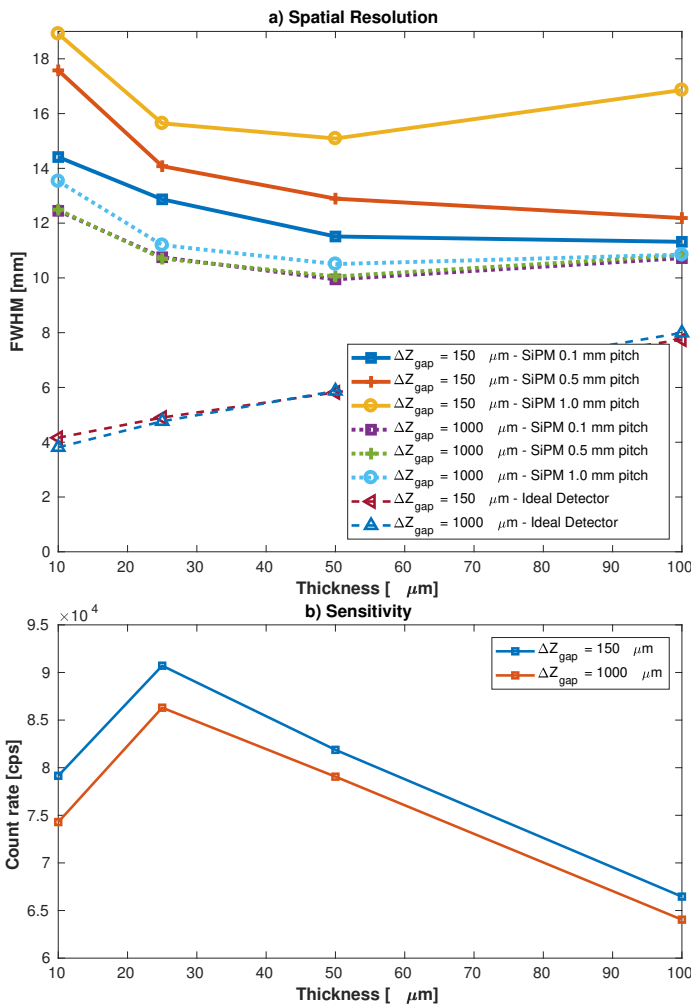
Fig. 14. Results for the simulations of a point source at 10 mm from the probe taking into account the optical photons generation and the SiPM readout, for probes with an air gap of 150 μm and 1000 μm and a SiPM with pixel pitch of 0.1, 0.5 and 1 mm. a) Spatial resolution in the backprojected images as a function of the scintillator thickness. b) Sensitivity as a function of the scintillator thickness and the air gap. The trade-off between spatial resolution and sensitivity can be observed.
