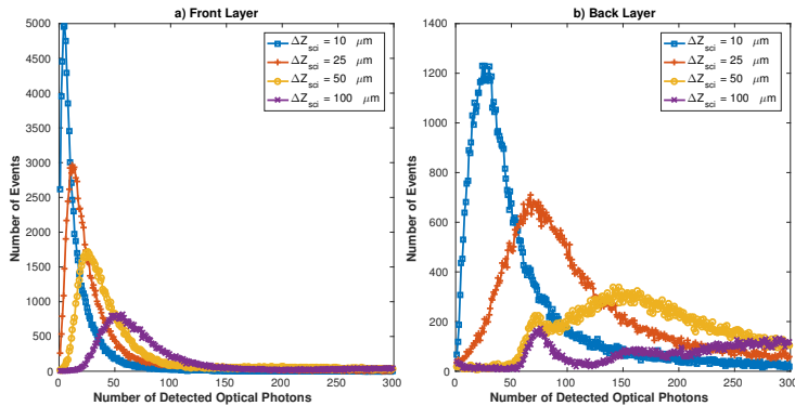
Fig. 15. a) Number of optical photons detected by the SiPM coming from the front layer for scintillator thicknesses of 10, 25, 50 and 100 μm. b) Number of optical photons detected by the SiPM coming from the back layer for scintillator thicknesses of 10, 25, 50 and 100 μm.
