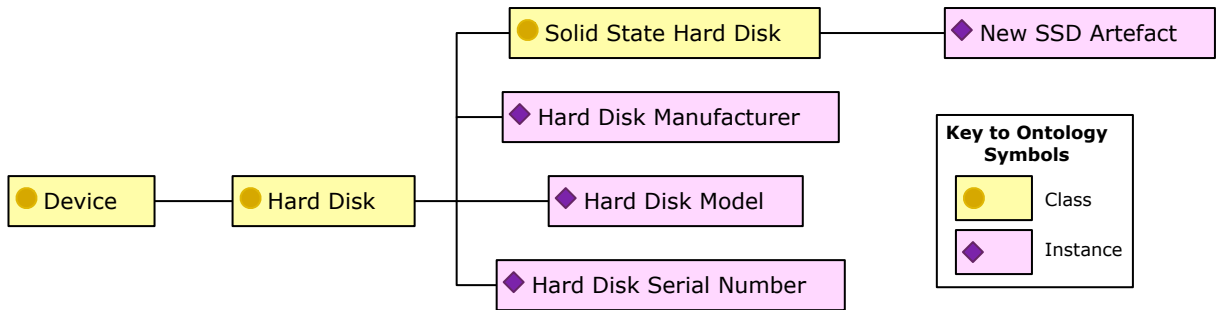
Fig. 4.7 Location Class: the addition of a sub-class for Solid State Devices
