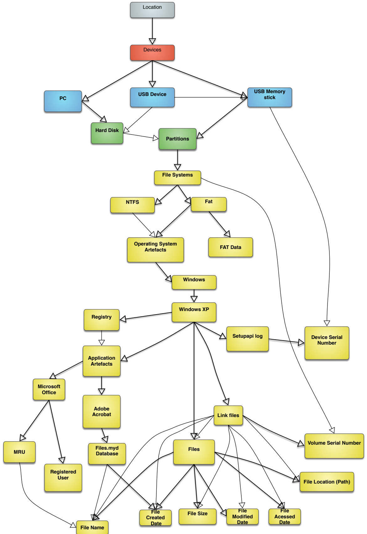
Fig. 4.2 A representation of artefacts as classes. Note the complexity as the various subclasses start linking to each other.
