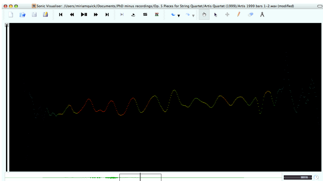
Figure 10: Artis Quartett (1999), G#, bar 2, cello, microintonation Sonic Visualiser peak frequency spectrogram. Sharpening intonation coupled with softening dynamic (shown by the colour change from orange through yellow to green).
