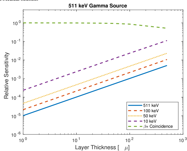
Fig. 2. Theoretical count rates in a plastic scintillator for collimated gamma sources of 511, 100, 50 and 10 keV and the coincidence count rate in a dual layer probe for a collimated \beta+ source ( ^{18}\text{F} ), both as a function of the scintillator thickness.
