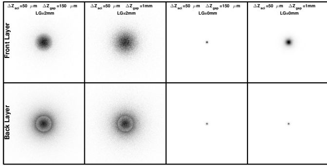
Fig. 13. Spatial distribution of optical photons on the SiPM surface obtained after the impact of 1 \times 10^4 positrons for different probe configurations with and without a light guide (LG).
