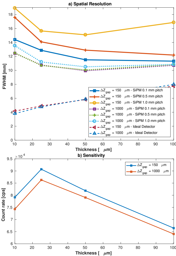
Fig. 14. Results for the simulations of a point source at 10 mm from the probe taking into account the optical photons generation and the SiPM readout, for probes with an air gap of 150 μm and 1000 μm and a SiPM with pixel pitch of 0.1, 0.5 and 1 mm. a) Spatial resolution in the backprojected images as a function of the scintillator thickness. b) Sensitivity as a function of the scintillator thickness and the air gap. The trade-off between spatial resolution and sensitivity can be observed.
