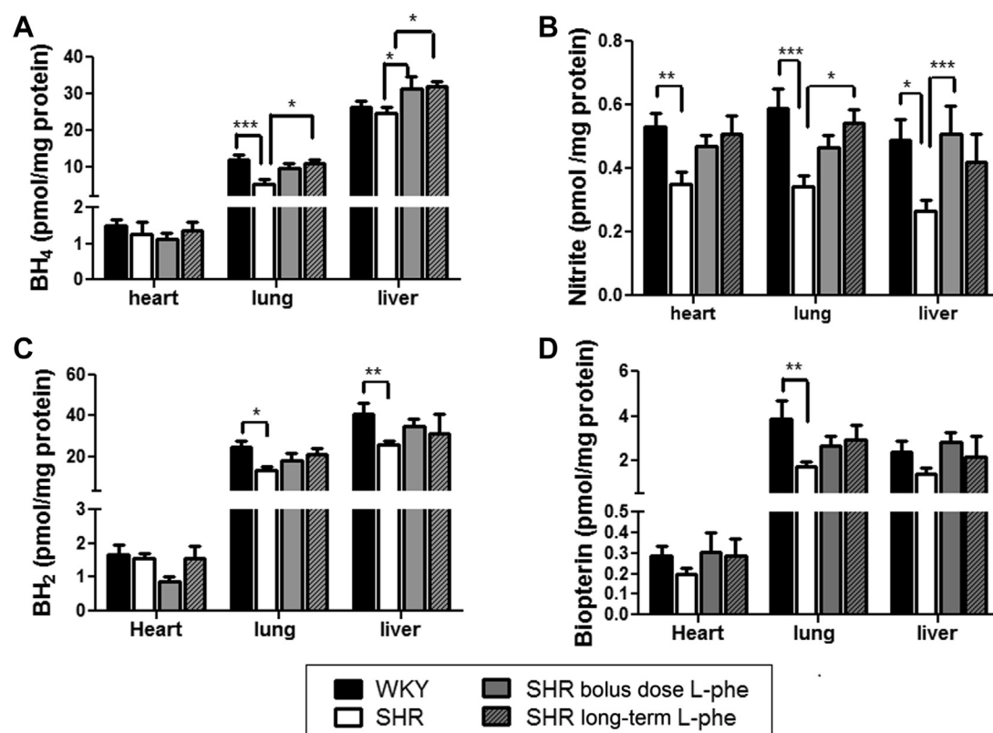
FIGURE 2 Effects of Short-Term and Long-Term L-Phe on Tissue BH 4 and Nitrite In Vivo
