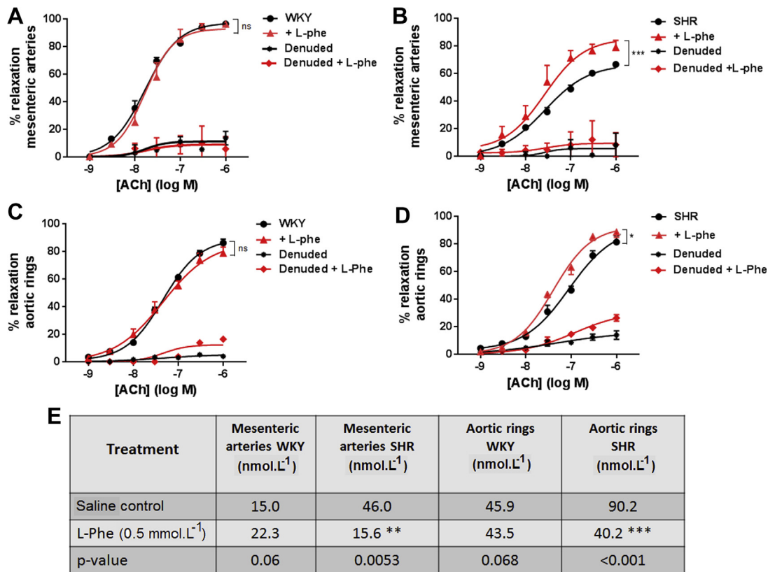
FIGURE 4 Effects of Short-Term L-Phe on Aortic and Mesenteric Vascular Reactivity
