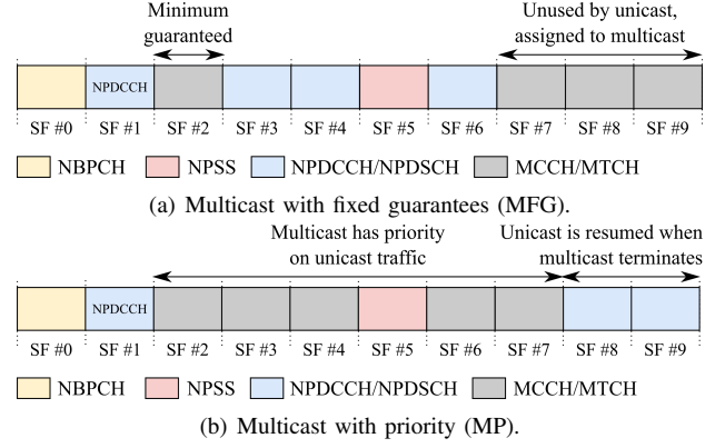
Fig. 6. Proposed transmission schemes applied to odd frames of NB-IoT.
