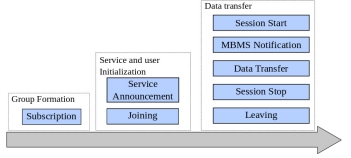
Fig. 4. Procedures for the reception of a MBMS service.
