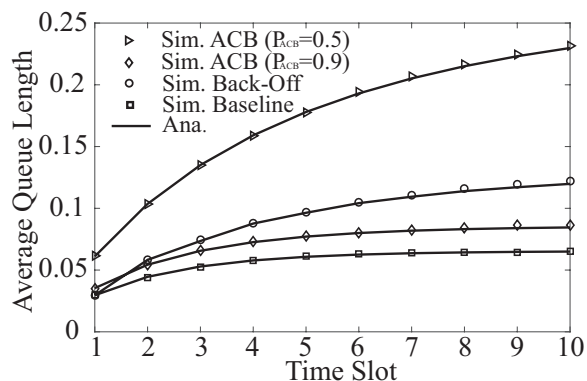
Fig. 8: Average Queue Length of each time slot.
