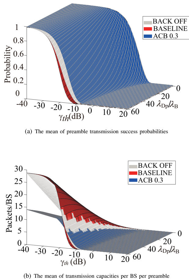
Fig. 10: The mean of preamble transmission success probabilities and the transmission capacities per BS per preamble
