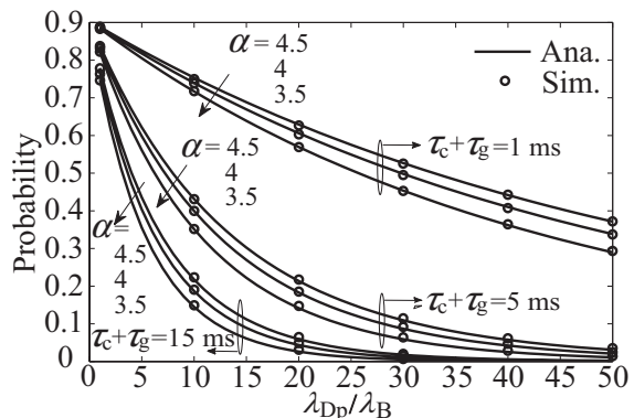
Fig. 5: Preamble transmission success probability.
