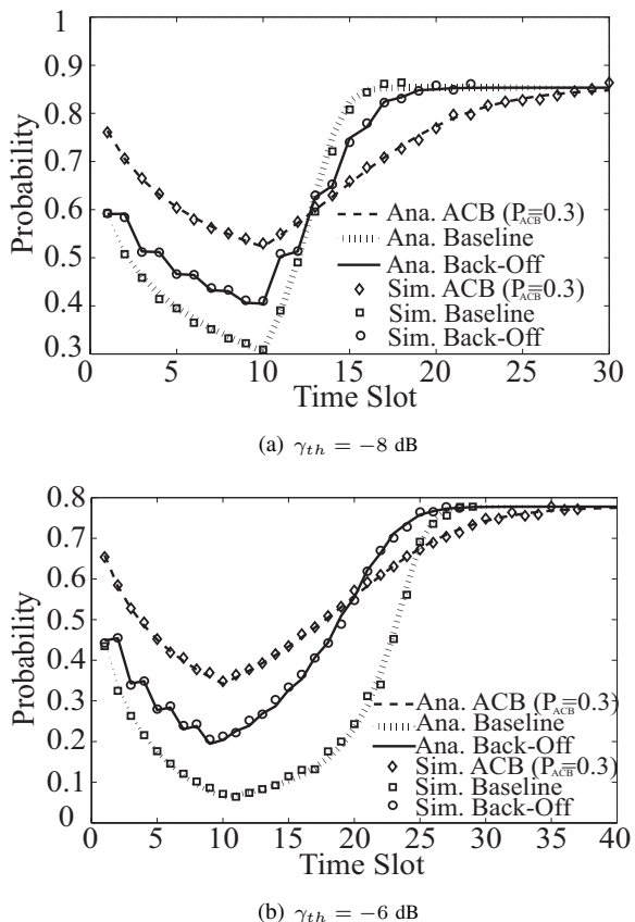
Fig. 9: Preamble transmission success probability of each time slot.
